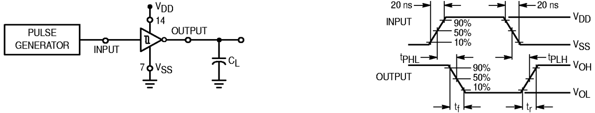
Figure 1. Switching Time Test Circuit and Waveforms
