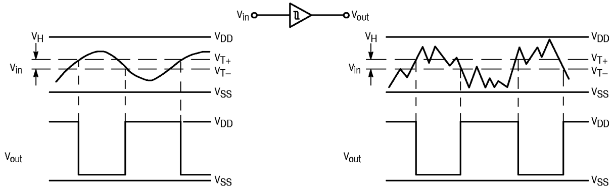
(a) Schmitt Triggers will square up inputs with slow rise and fall times.
