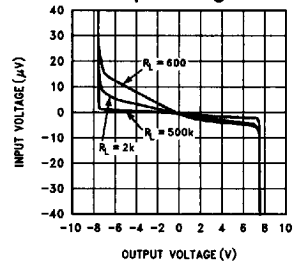
Input Voltage vs Output Voltage
