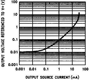
Output Characteristics Sourcing Current
