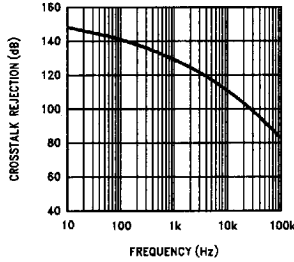
Crosstalk Rejection vs Frequency
