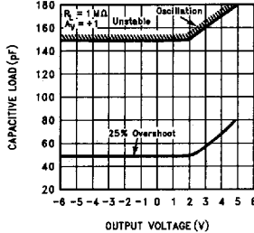
Stability vs Capacitive Load R_L = 1M\Omega
