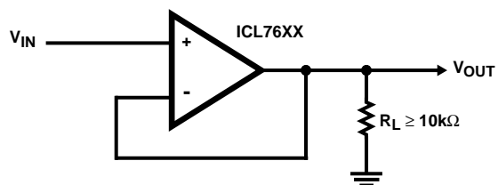
FIGURE 1. SIMPLE FOLLOWER
